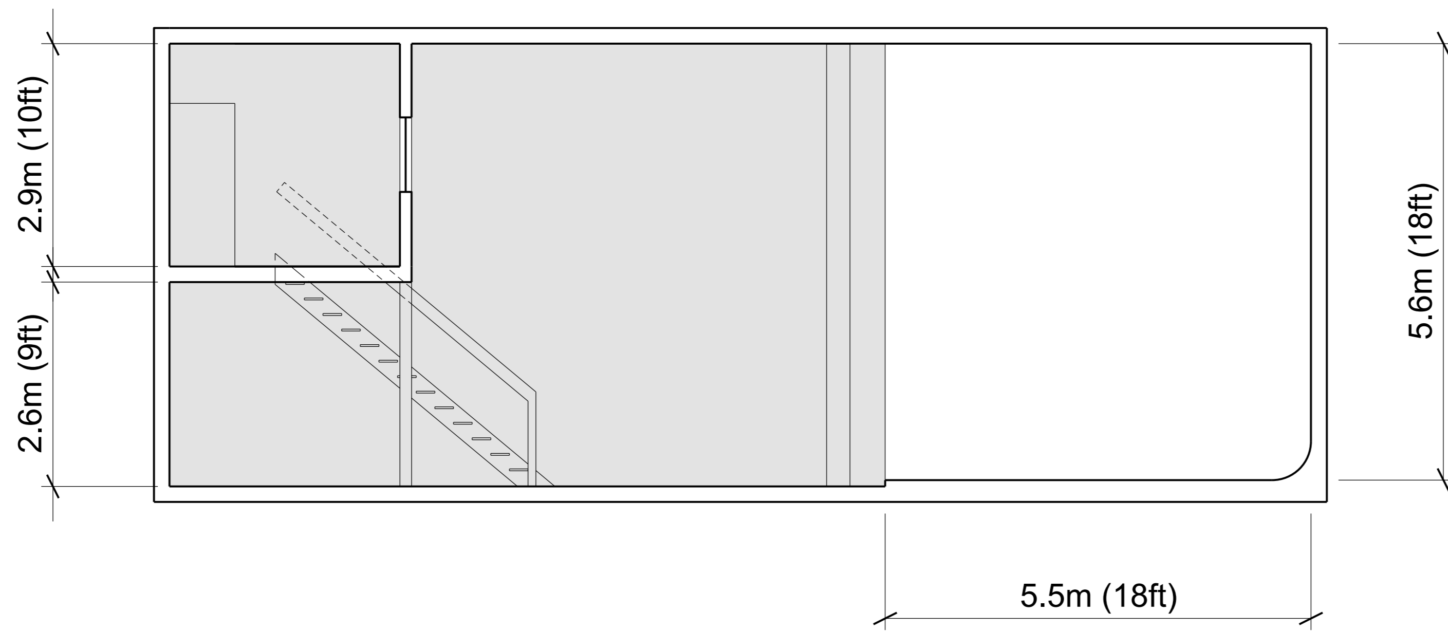
Section AA
