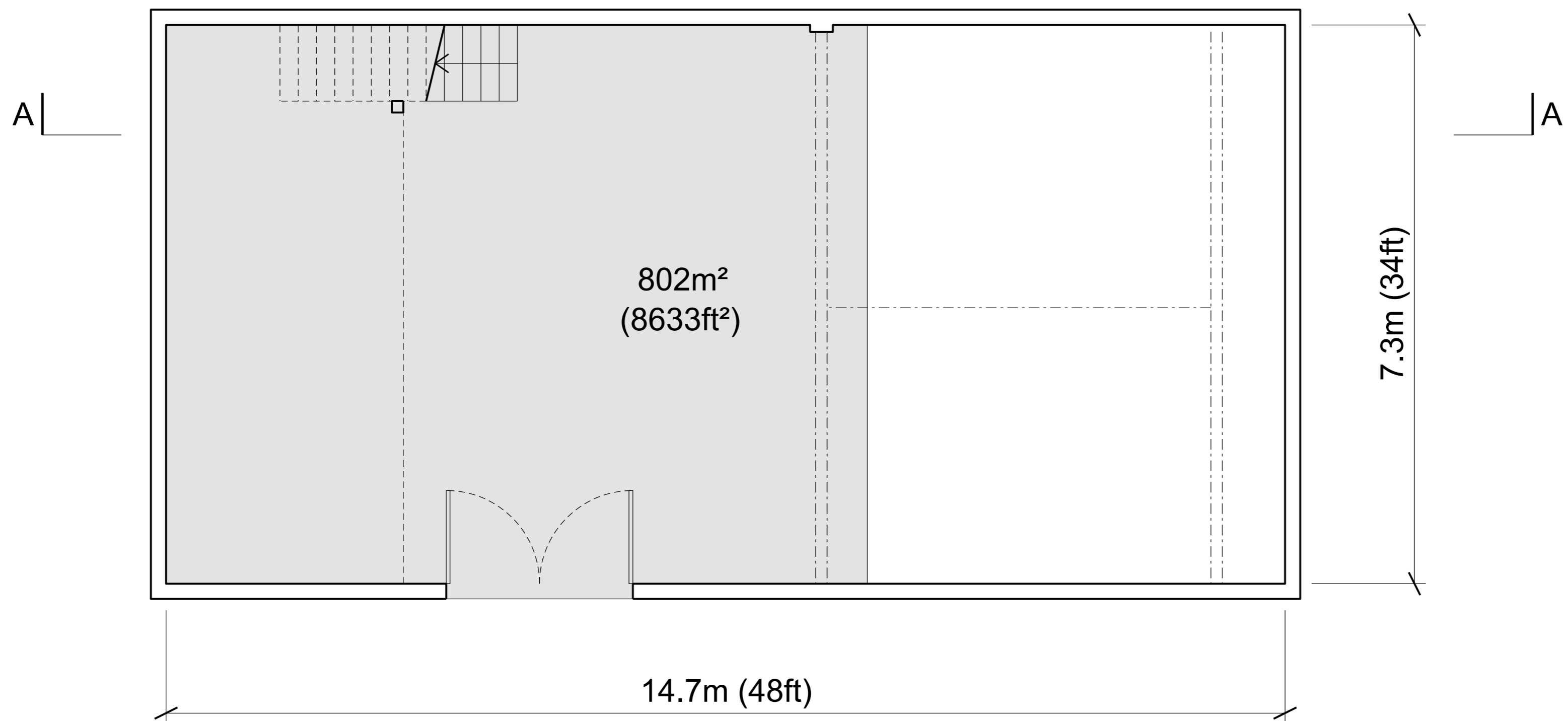
Plan
