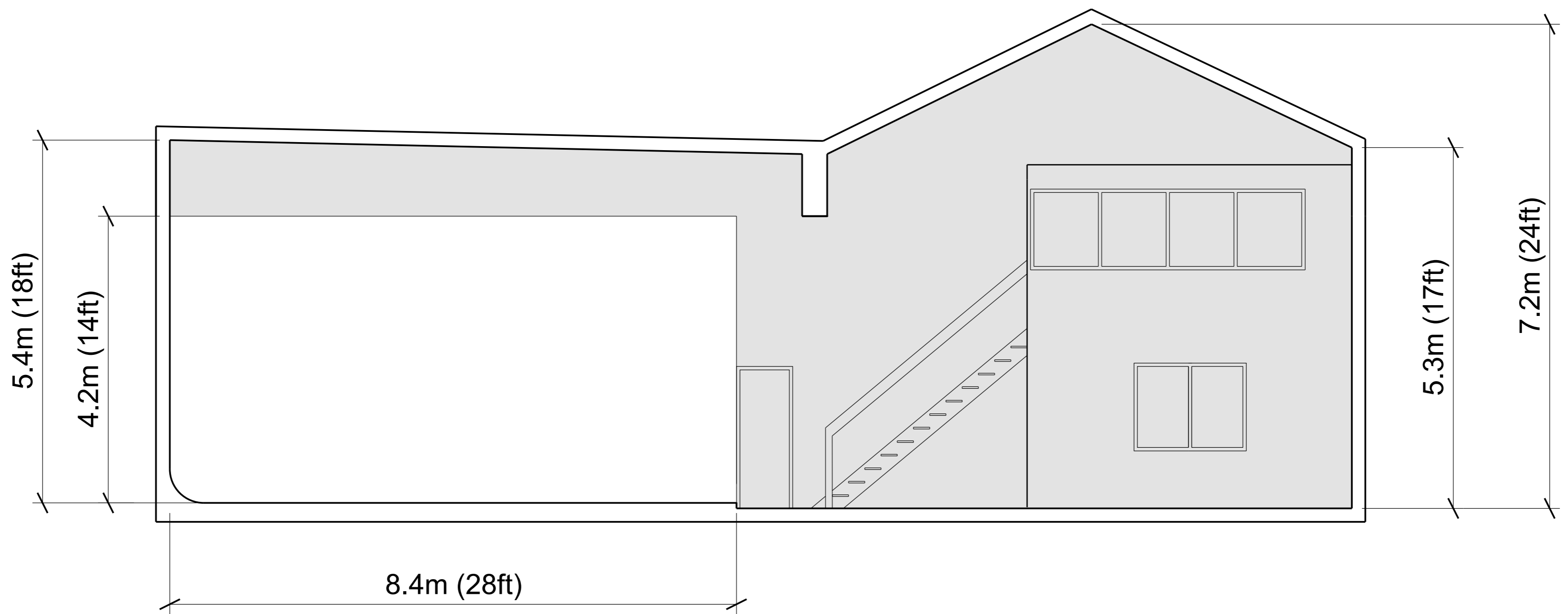
Section AA
