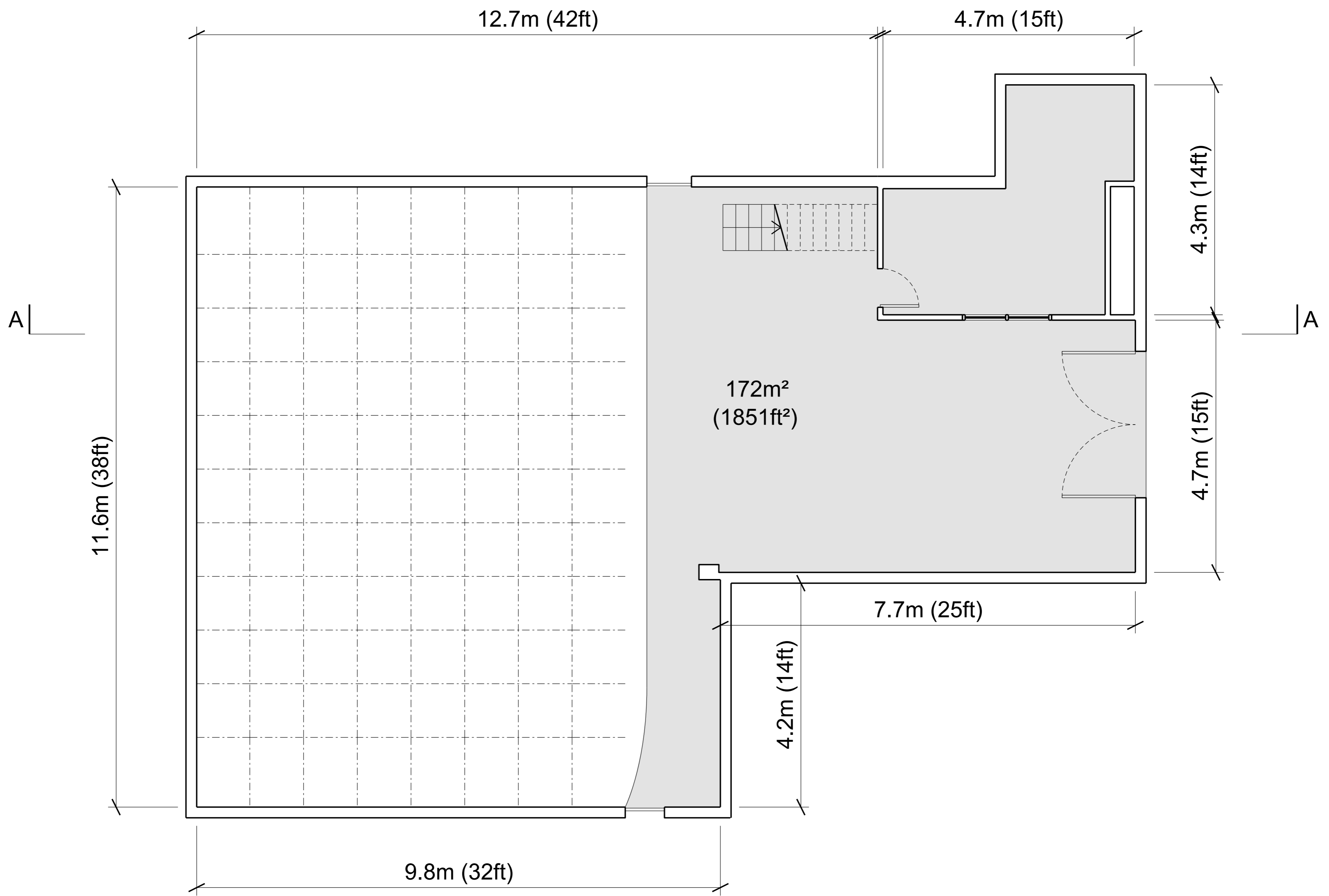
Plan
