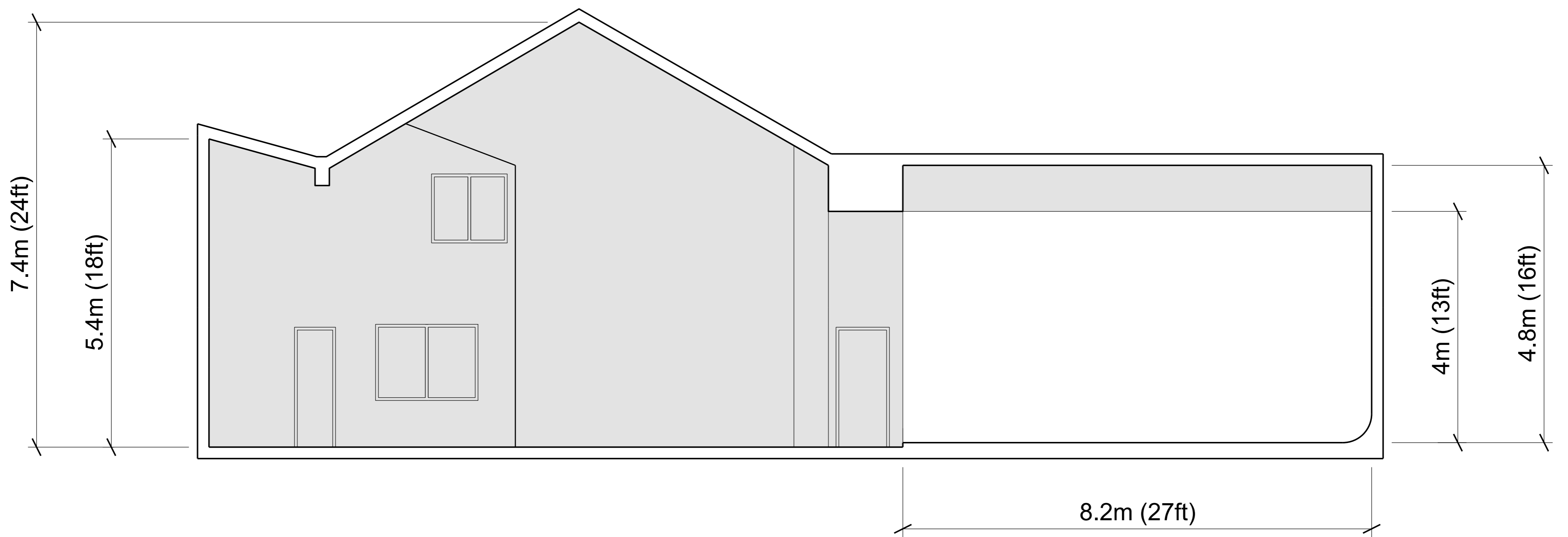
Section AA
