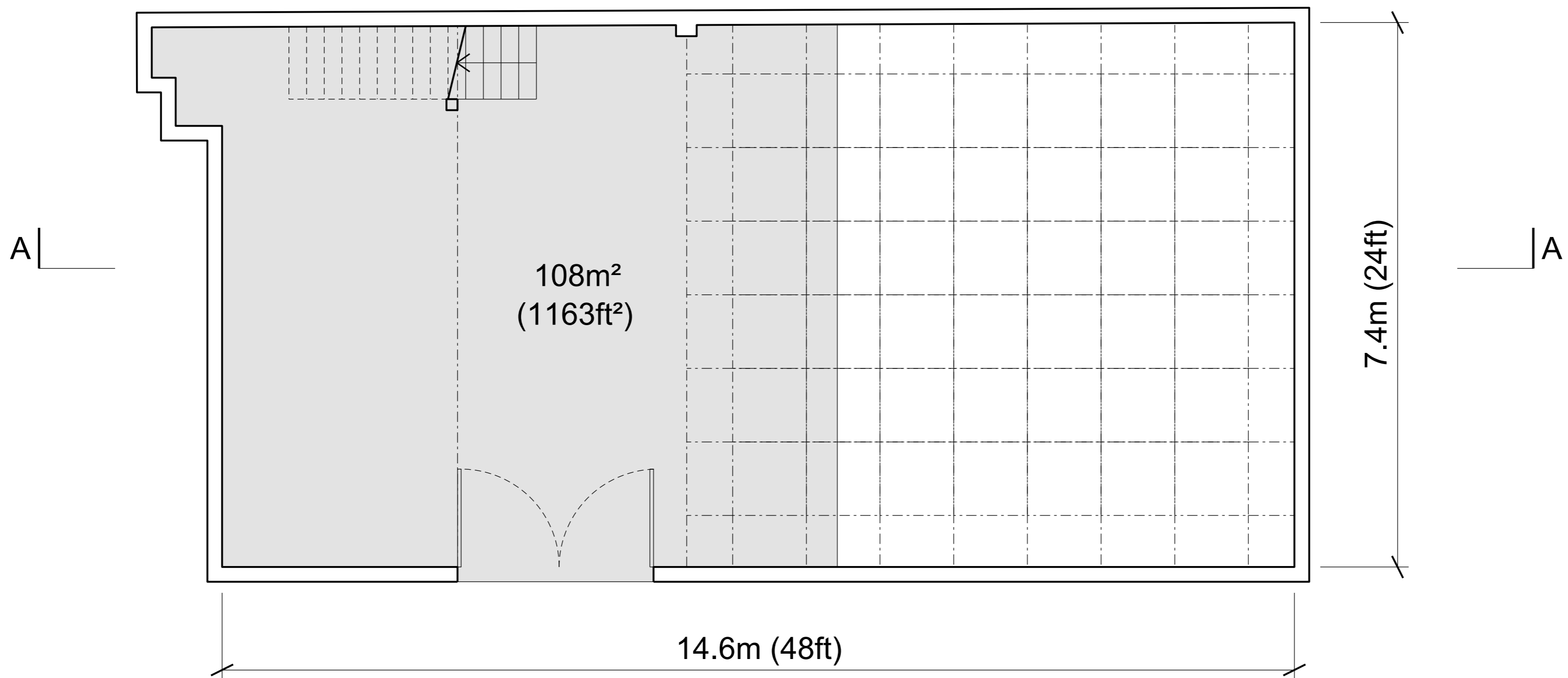
Plan
